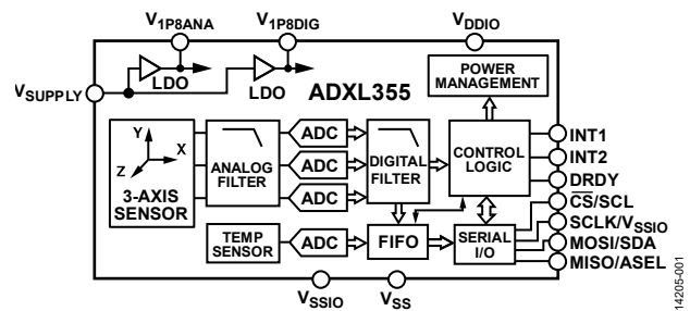
Figure 2. ADXL355
